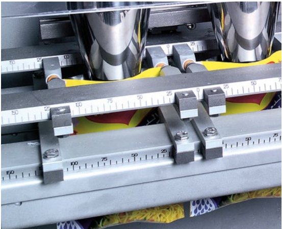
Wide sachet opening, enabling higher filling grade.
