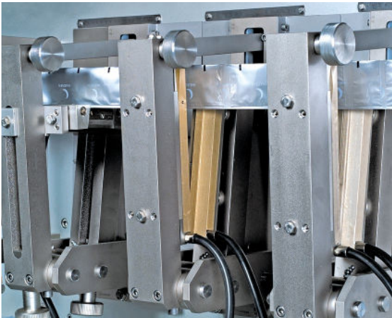
This model in duplex version includes two independent vertical sealing groups.
